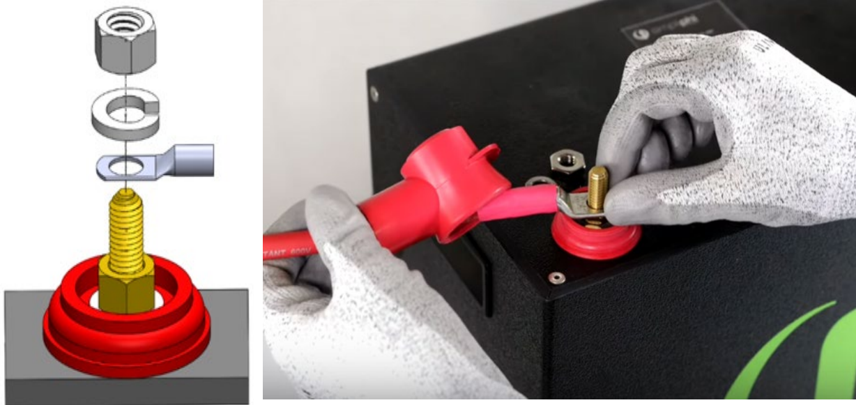
Figure 7.0 – Cable Lug Wiring onto AmpliPHI Threaded Stud
