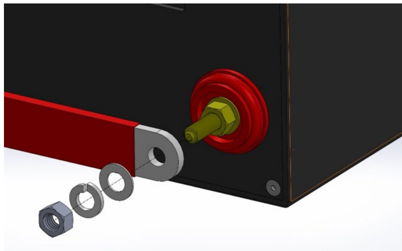
Figure 9.0 – Interconnecting Busbar Wiring onto AmpliPHI Threaded Stud
