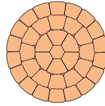
37 Strands Compact
