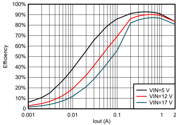
Figure 5-13. TPS562206 Efficiency at 1.05 Vout With 2.2uH Inductor
