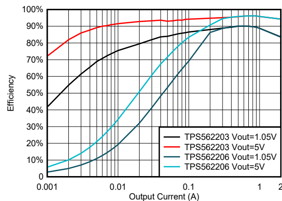
TPS562203 and TPS562206 Efficiency
